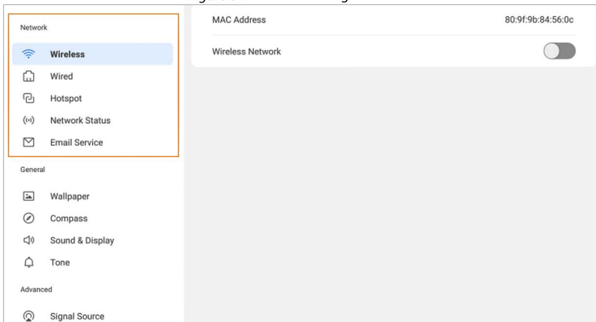
Figure 6-1 Network settings
