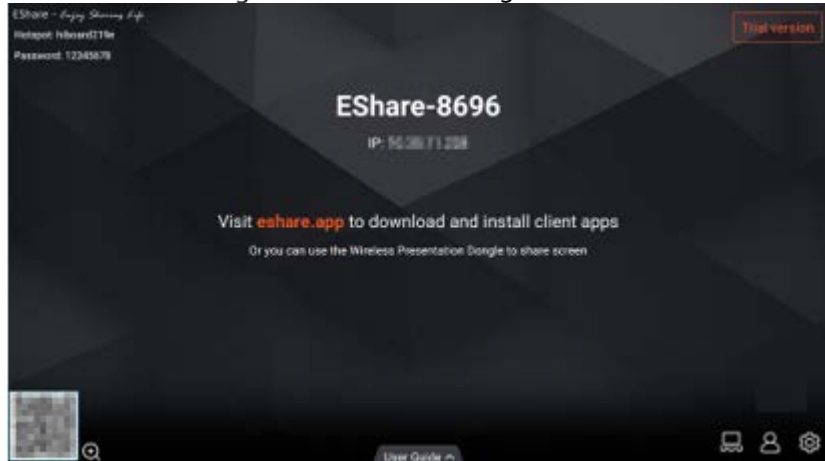
Figure 5-7 Screen Sharing
