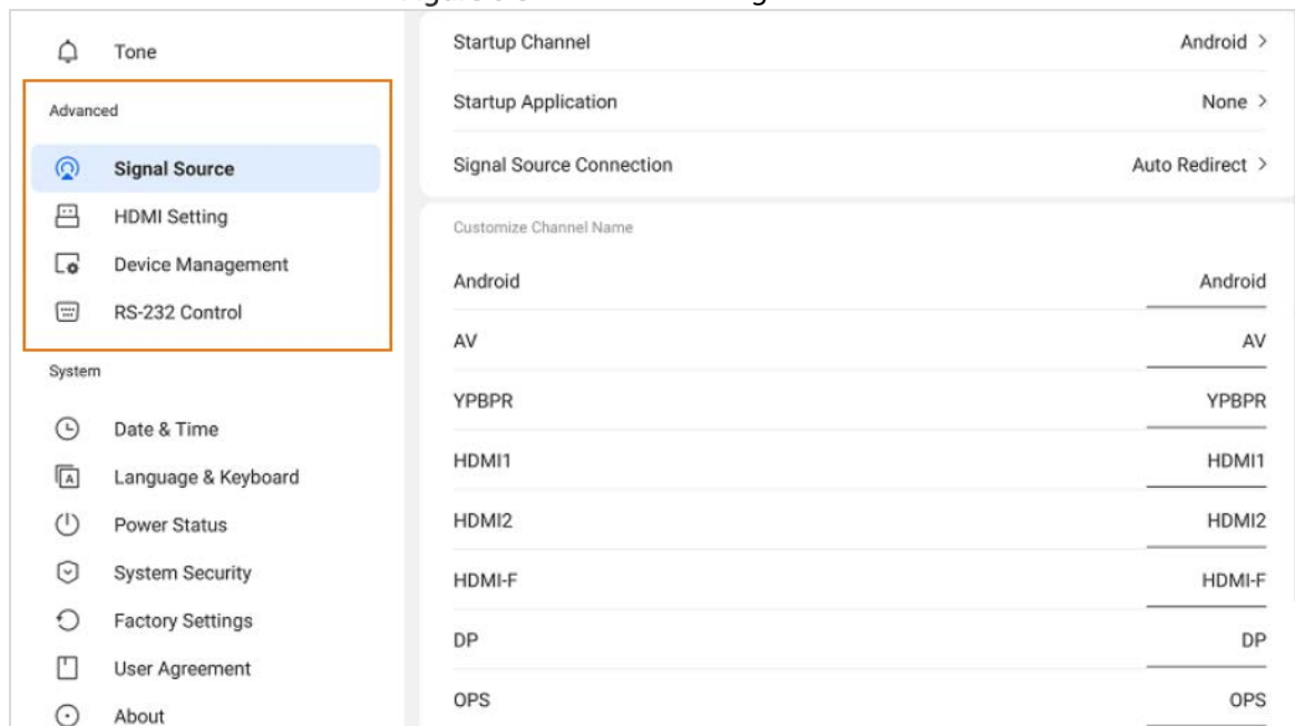
Figure 6-3 Advanced settings
